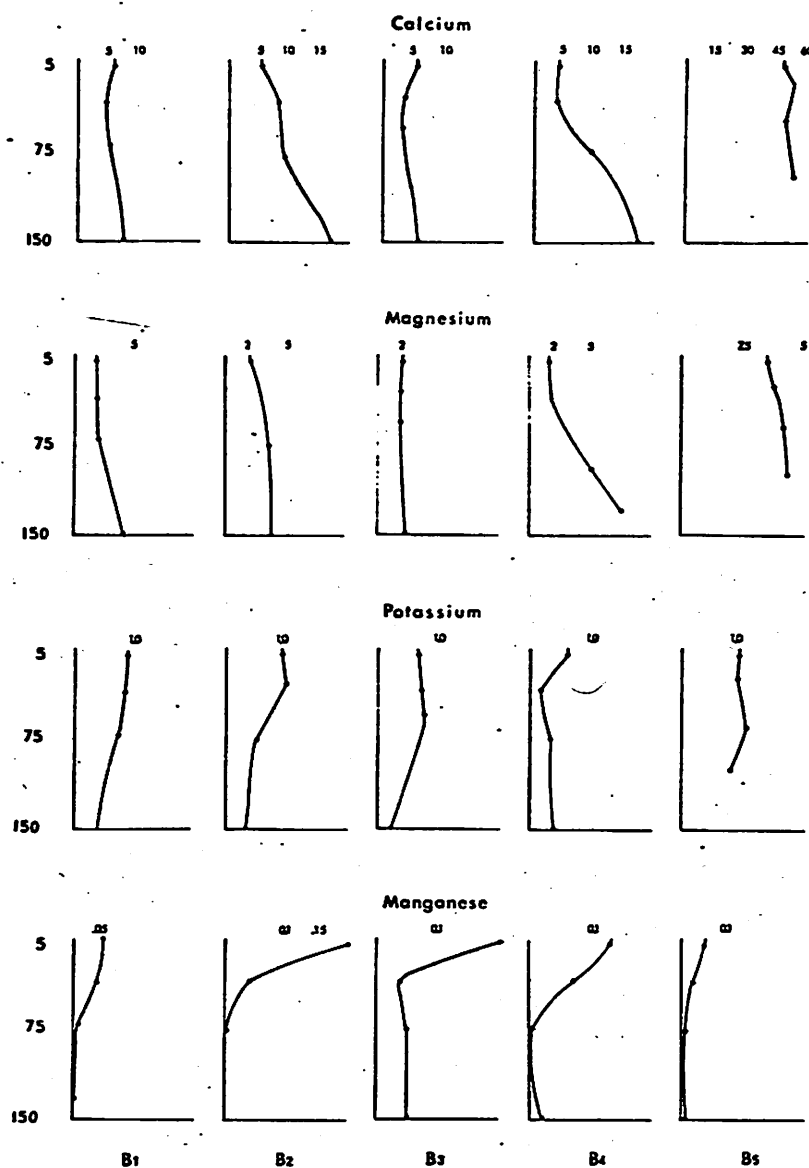
Fig. 4. A typical array of exchangeable cation profiles with respect to profile depth and topographic location. The vertical axis of each tier represents profile depth in centimeter, while the horizontal axis represents the exchangeable cation level measured as milliequivalents per 100 g of soil. The five graphs of each tier correspond to the five profiles sampled in the B catena near the Mbula study area. B 1 was a typical aridisol highest on the slope, while B 5 represents the vertisolic clay of the valley bottom.
