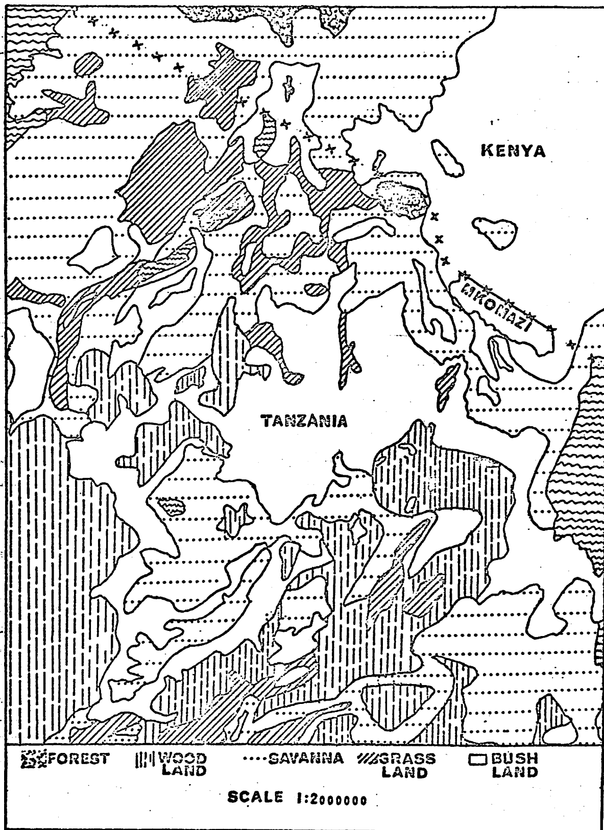
Fig. 5. The major vegetation types of northern Tanzania and southern Kenya. The Mkomazi Reserve is contained in the type known as bush, bushland, or "nyika." Redrawn from the Division of Overseas Survey D.O.S. 299E.
